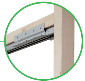
Reversible brackets convert 2 singles into a double
