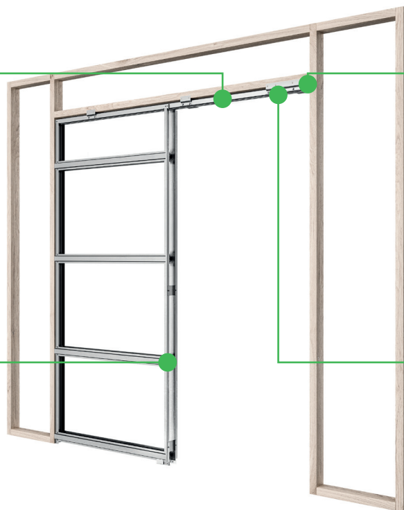
Full galvanized steel pocket system adjusts to 5 different door widths
